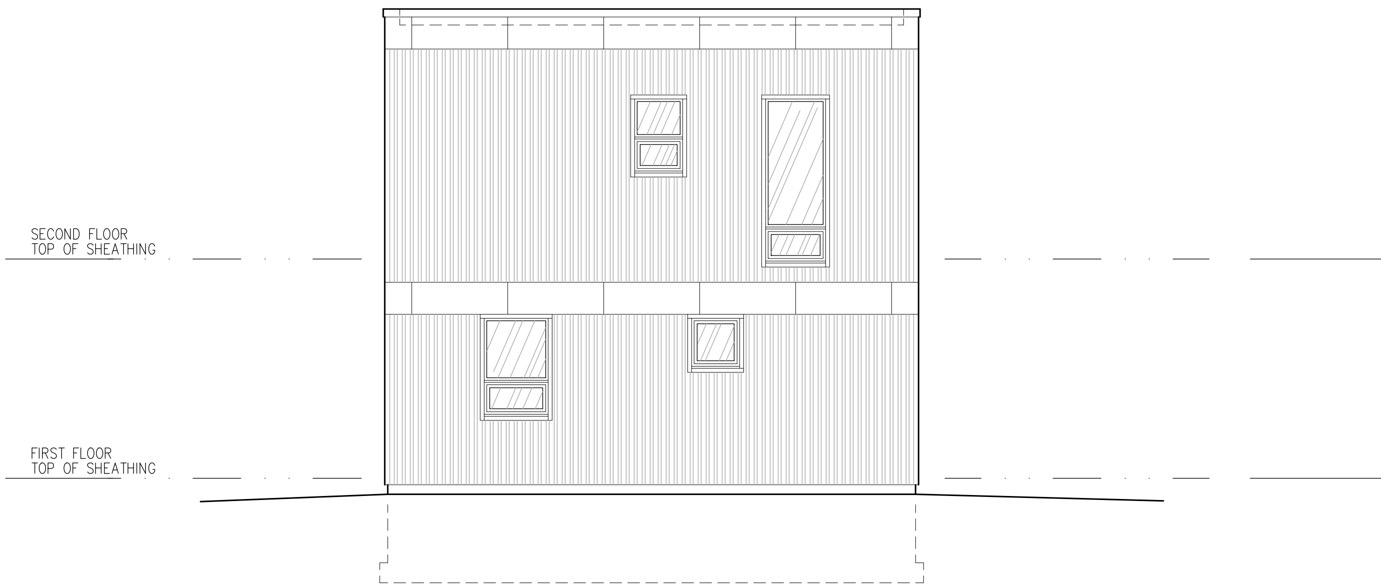
East Elevation BUILDING C
