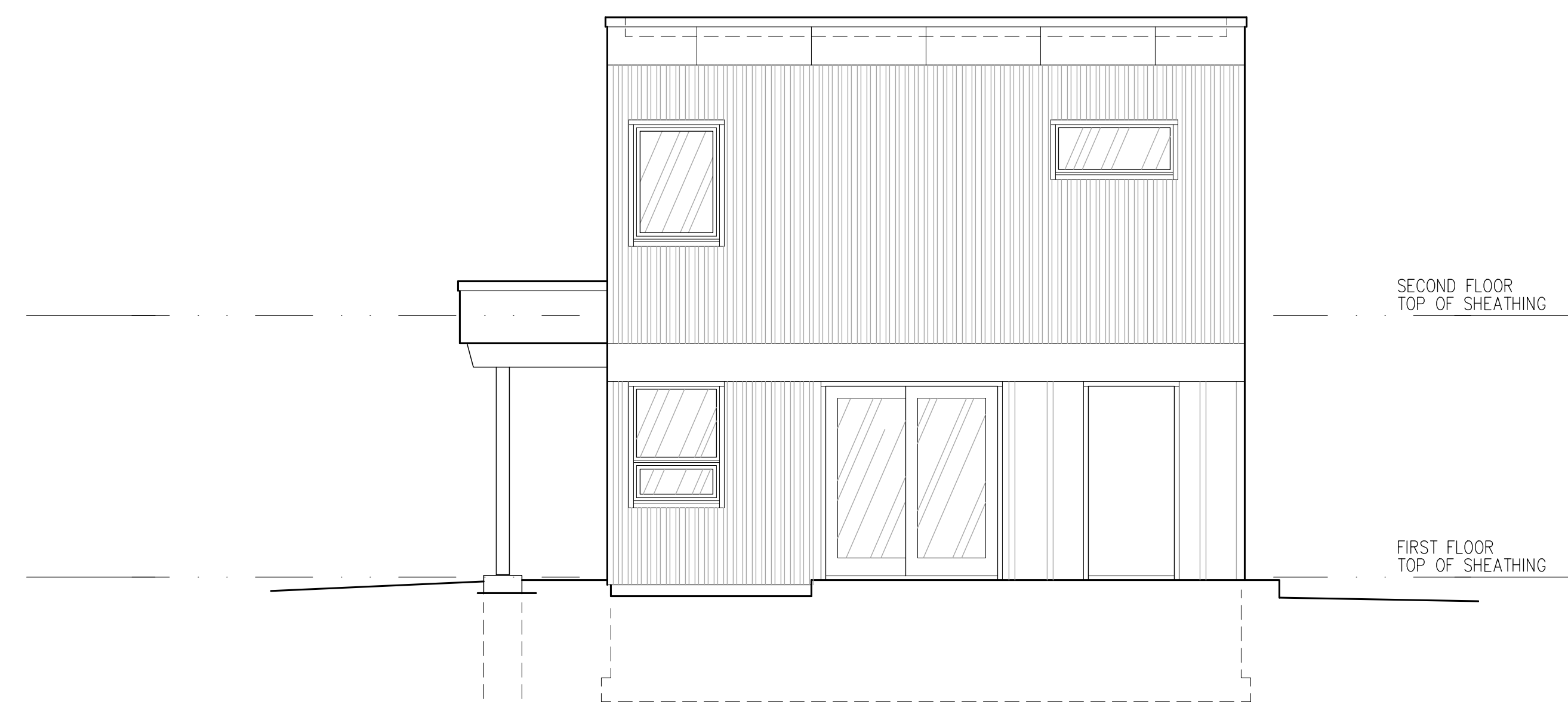
South Elevation BUILDING C
