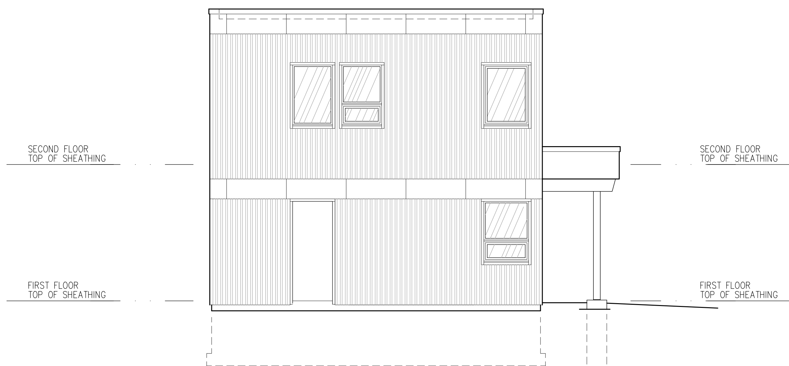
North Elevation BUILDING C
