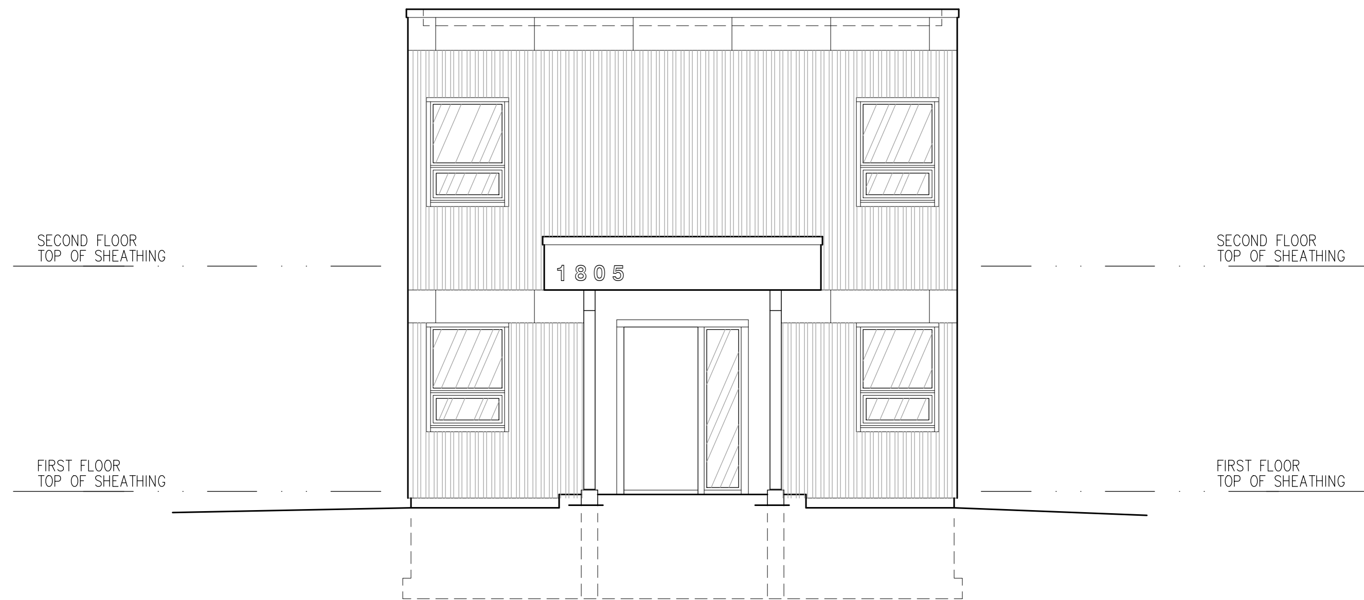
West Elevation BUILDING C
